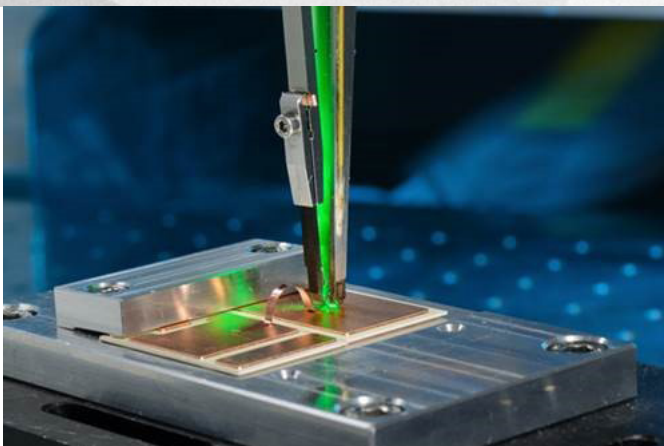
Image of the experimental set-up. The metal ceramic substrate lays on the sample holder, while a copper band is laser-welded on it. The laser is located on top of the sample and aimed at the copper band. (Credit: Fraunhofer ILT)
